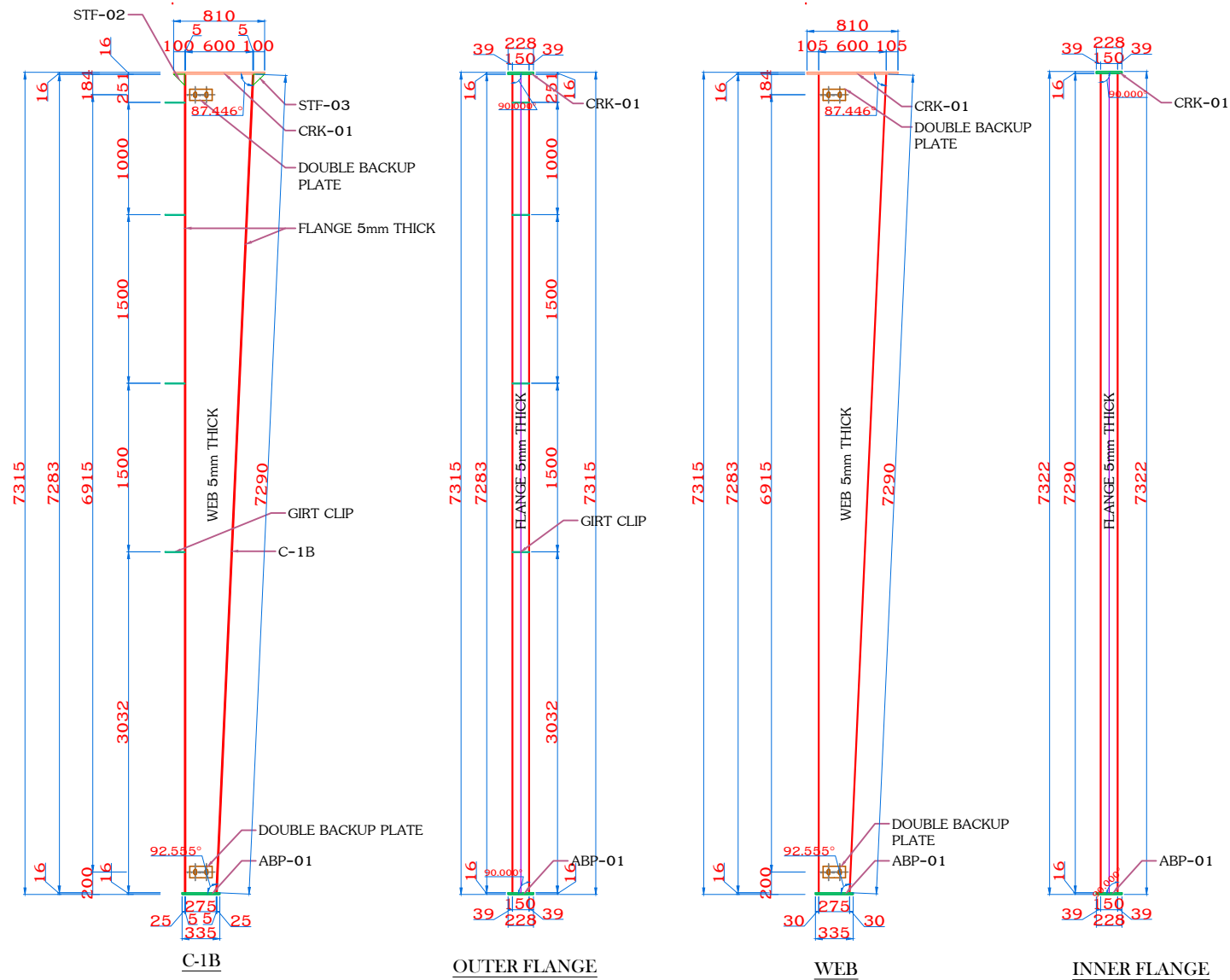
COLUMN DETAIL C-1B @ GRID 2 TO 4 QTY:(03,L)(03,R)
